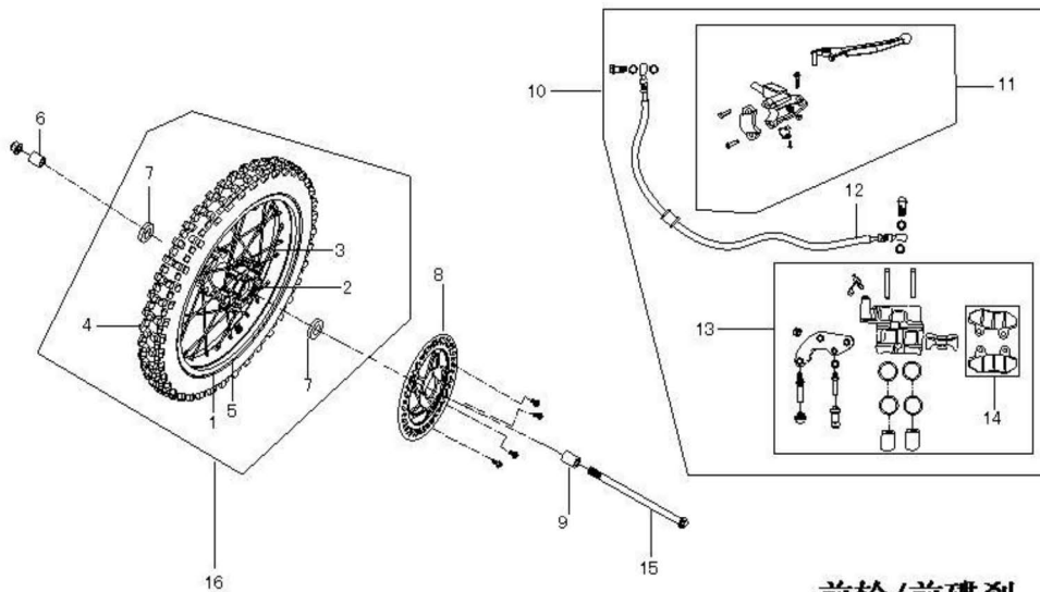
前轮/前碟刹 FT. WHEEL / BRAKE ASSY
