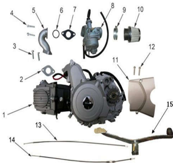
汽油机总成 /ENGINE ASSY.
